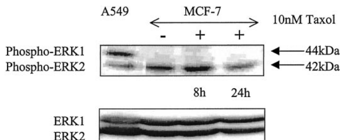
Fig. 6. Expression of ERK and phospho-ERK in paclitaxel (Taxol)-treated MCF-7 cells. Cells were treated with 10 nM paclitaxel for the indicated times and 20 \mu g of total cell lysate was used for immunoblot analysis, together with 20 \mu g of total cell lysate from A549 cells. Compared with A549 cells, MCF-7 cells expressed low levels of phospho-ERK and did not exhibit paclitaxel-induced ERK activation.
